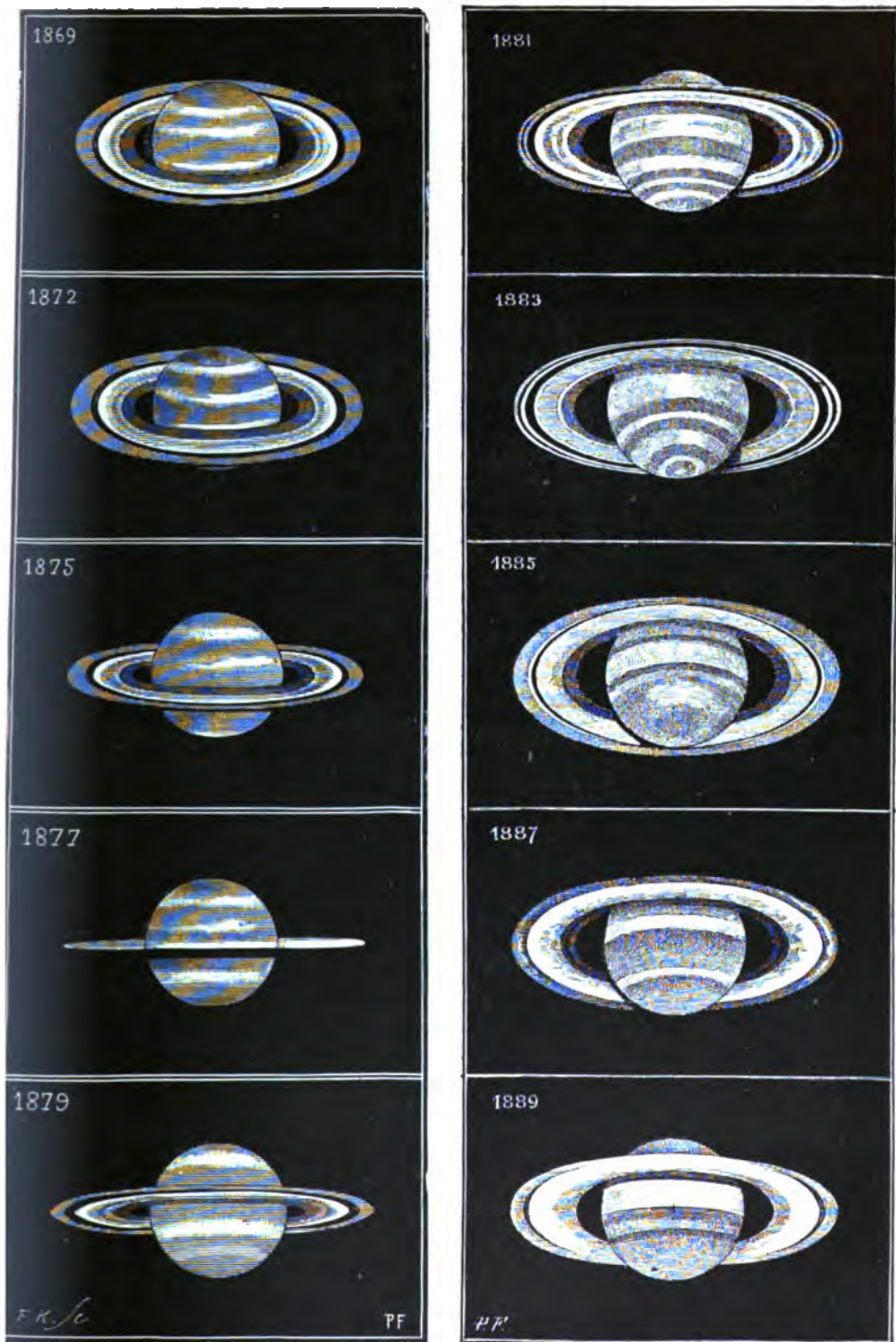
FIG. 189.—CHANGES IN APPEARANCE OF SATURN'S RINGS
