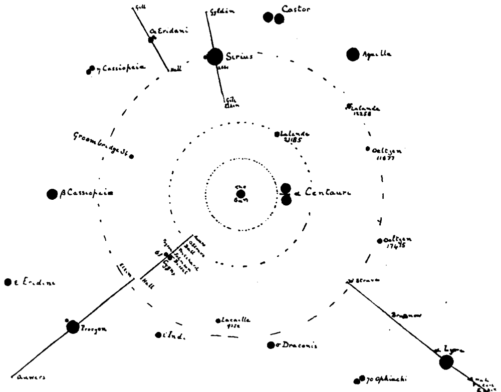
FIG. 261.—DIAGRAM BY MR. A. C. RANYARD, SHOWING THE DISTANCES OF TWENTY STARS FOR WHICH LARGE PARALLAXES HAVE BEEN FOUND. (From Knowledge , June 1, 1889.)
