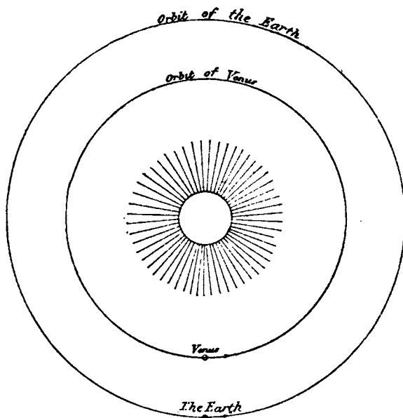
FIG. 90.—ORBITS OF VENUS AND OF THE EARTH AROUND THE SUN
