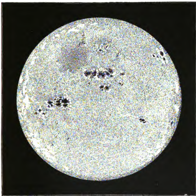
FIG. 99.—THE SUN. (From a direct Photograph)
