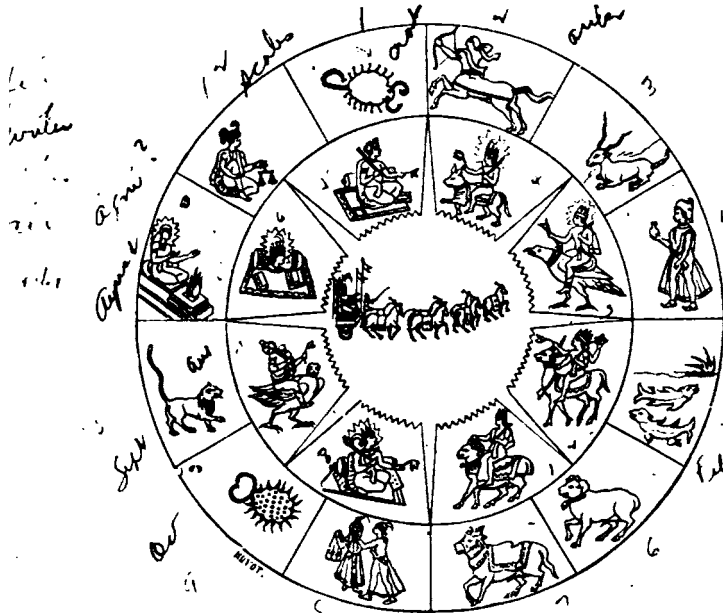
FIG. 252.—ANCIENT HINDOO ZODIAC
