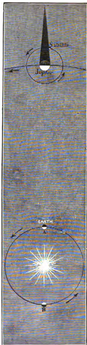
FIG. 139.—ECLIPSE OF ONE OF JUPITER'S SATELLITES
