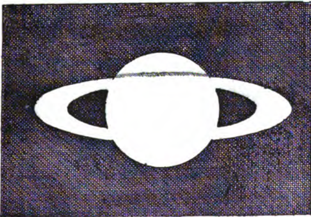
FIG. 186.—FIRST DRAWING OF SATURN'S RING, MADE BY HUYGENS IN 1657
