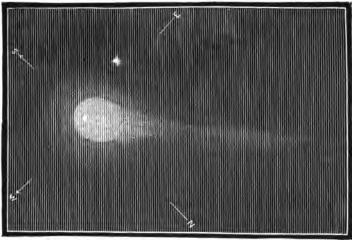
FIG. 212.—THE COMET OF PONS 1812, WHICH RETURNED IN 1883
