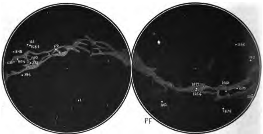
FIG. 266. — POSITION IN THE HEAVENS OF TEMPORARY STARS
