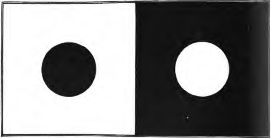
FIG. 103.—EFFECT OF IRRADIATION
