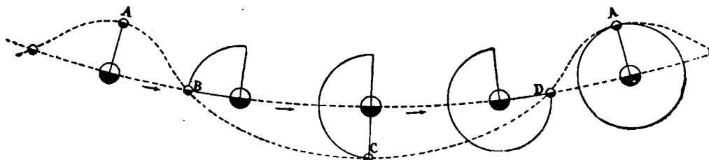
FIG. 41.—COMBINED MOVEMENT OF THE EARTH AND MOON
