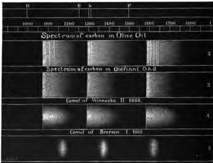
FIG. 226.—SPECTROSCOPIC ANALYSIS OF COMETS
