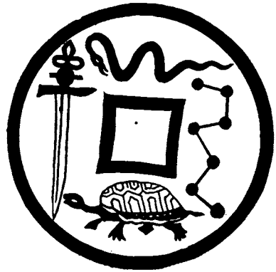
FIG. 254.—CHINESE MEDAL, SHOWING THE GREAT BEAR
