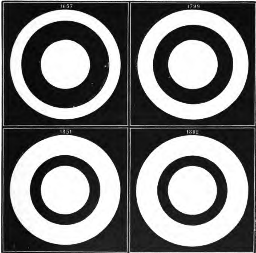
FIG. 192.—PROBABLE DRAWING TOGETHER OF SATURN'S RINGS SINCE THEIR DISCOVERY
