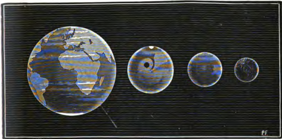
FIG. 168.—COMPARATIVE MAGNITUDES OF THE EARTH, MARS, MERCURY, AND THE MOON
