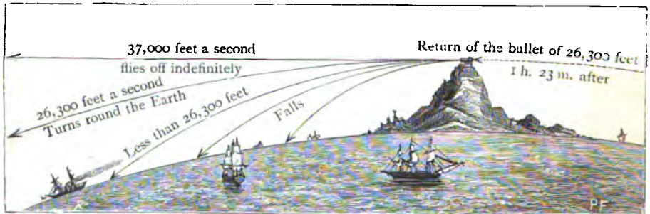
FIG. 58.—SPEED THAT IT WOULD BE NECESSARY FOR A PROJECTILE TO ATTAIN IN ORDER THAT IT SHOULD NEVER RETURN TO THE EARTH
