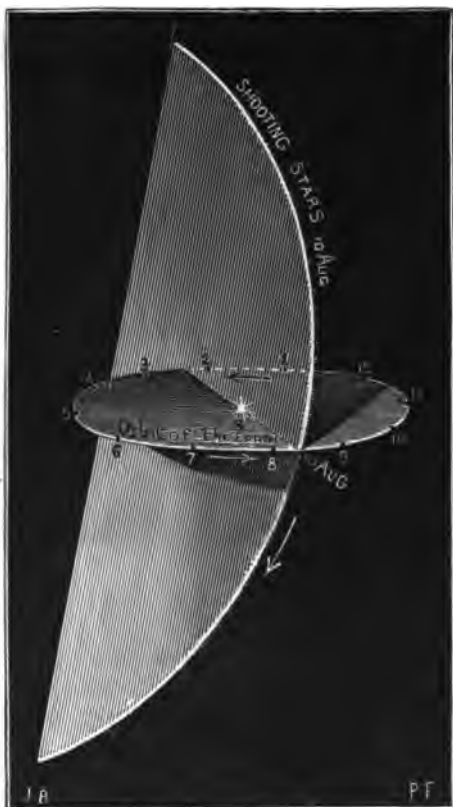
FIG. 232.—INTERSECTION OF THE ORBIT OF THE SHOOTING STARS OF AUGUST 10 WITH THE PLANE OF THE EARTH'S ORBIT
