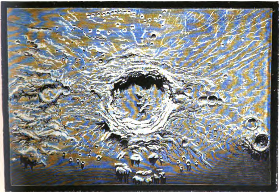
FIG. 48.—THE LUNAR CRATER COPERNICUS. (From a Drawing by Nasmyth)
