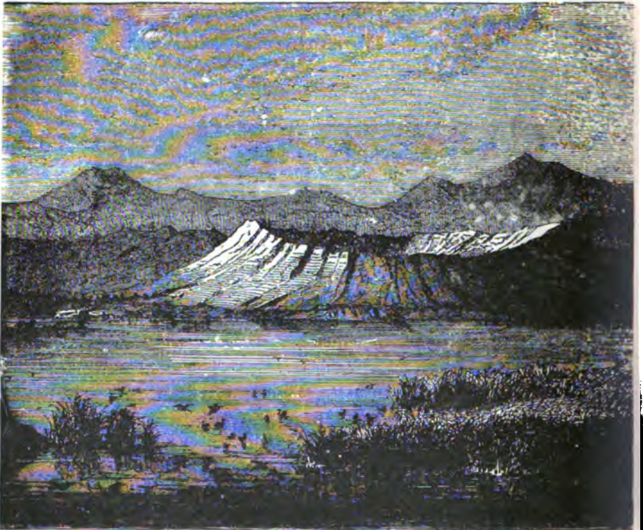
FIG. 52.—AN EXTINCT CRATER IN ICELAND: IMAGE OF A LUNAR LANDSCAPE BEFORE THE DISAPPEARANCE OF WATER
