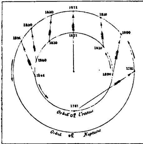
FIG. 201.—DISTURBANCES OF URANUS BY NEPTUNE
