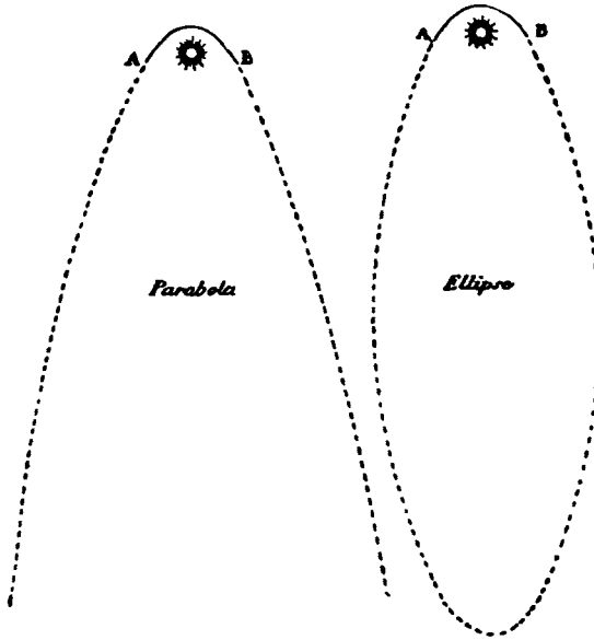
FIG. 207. — PARABOLA AND ELLIPSE
