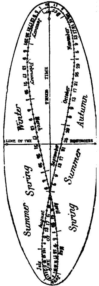
FIG. 7.—DETAILS OF THE MERIDIAN
