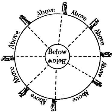
FIG. 21.—ALL OVER THE GLOBE, WEIGHT IS DIRECTED TOWARDS THE CENTRE
