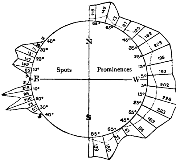
FIG. 123.—RELATIVE DISTRIBUTION OF SOLAR SPOTS AND PROMINENCES
