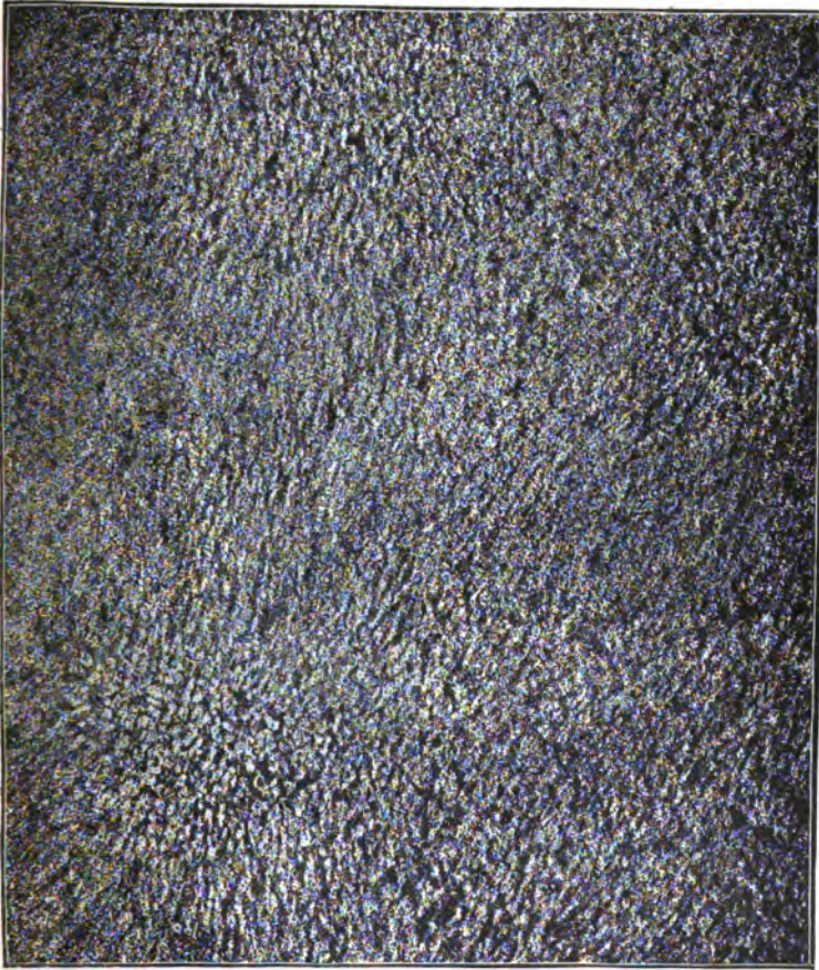
FIG. 102.—DIRECT PHOTOGRAPH OF THE SURFACE OF THE SUN, SHOWING LUMINOUS WAVES AND CURRENTS
