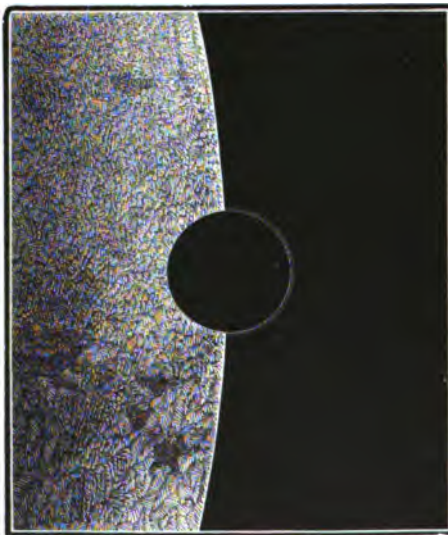
FIG. 164.—THE ATMOSPHERE OF VENUS ILLUMINATED BY THE SUN, AT THE MOMENT OF ENTRY UPON THE EDGE OF THE SUN
