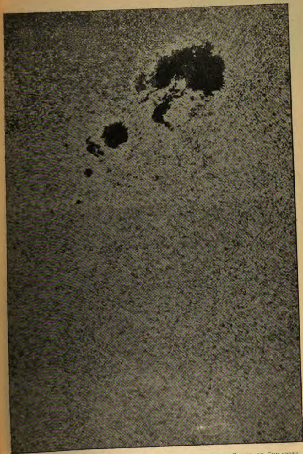
FIG. 134.—A PORTION OF THE SURFACE OF THE SUN, SHOWING A GROUP OF SUN-SPOTS AND RICE-GRAIN STRUCTURE OF THE PHOTOSPHERE. (From a Photograph taken at Meudon, by Dr. Janssen, June 1, 1881)
