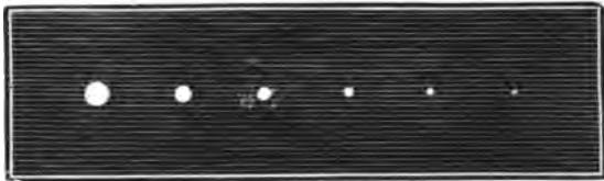
FIG. 257.—RELATIVE BRILLIANCY OF STARS OF THE FIRST SIX MAGNITUDES. (THE SURFACE OF THE DISCS IS PROPORTIONATE TO THEIR BRILLIANCY.)
