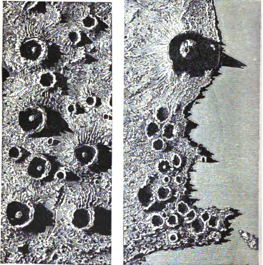
A Volcanic District—The Moon
