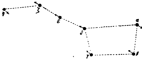
FIG. 268.—THE SEVEN STARS OF THE GREAT BEAR AS THEY REALLY ARE
