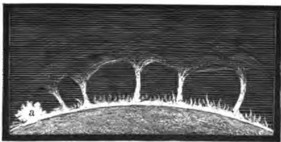
FIG. 117.—AN EXPLOSION IN THE SUN: FIRST PHASE
