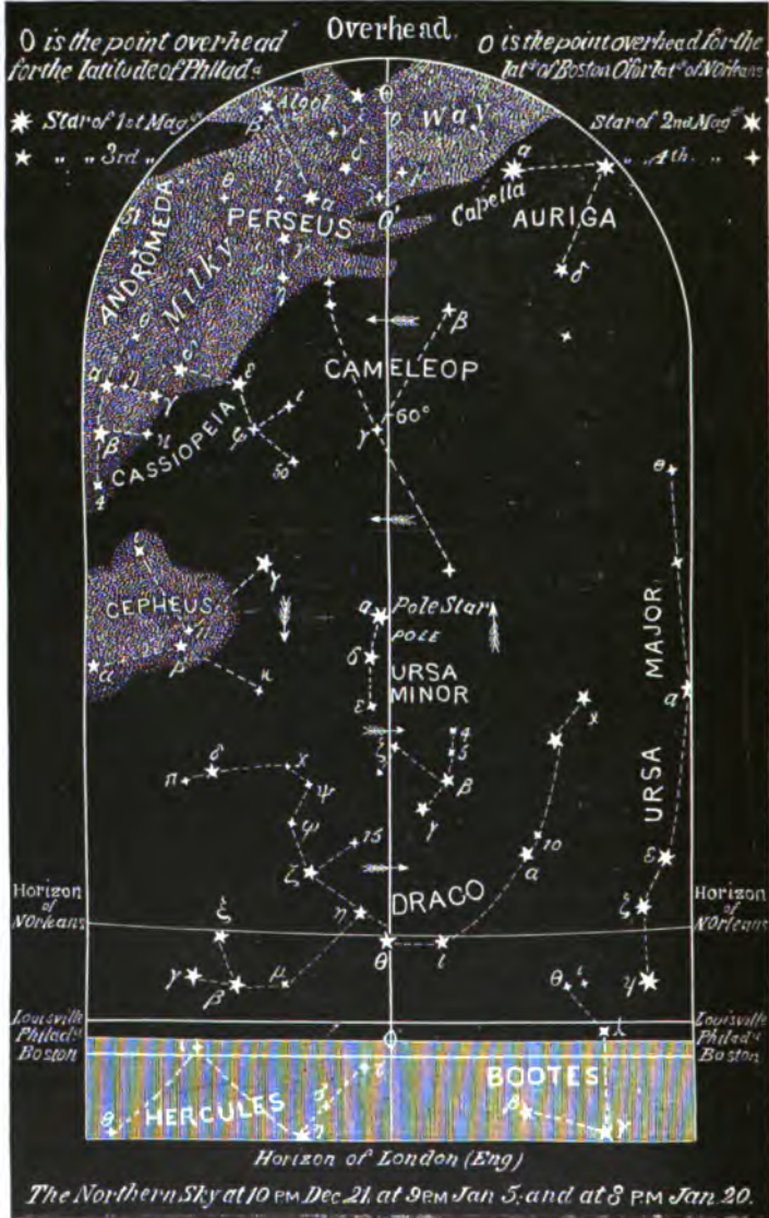
FIG. 13.—STARS SURROUNDING THE POLE, AND WHICH NEVER SET IN ENGLAND
