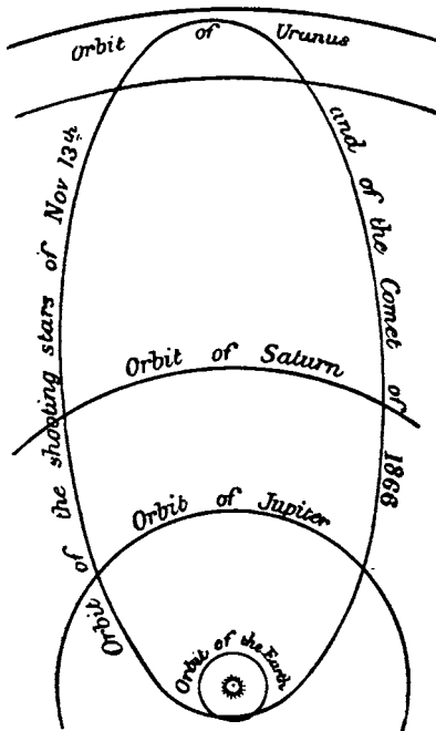
FIG. 210.—URANUS, THE COMET OF 1866, AND THE SWARM OF SHOOTING STARS OF NOVEMBER 13 Scale: 4 millimetres = 1 radius of the Earth's orbit
