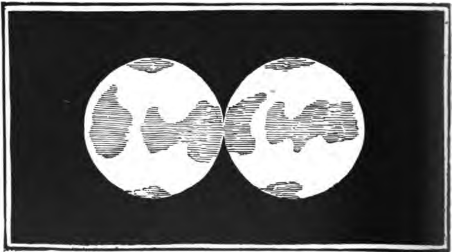
FIG. 166.—ROUGH SKETCH OF THE GEOGRAPHICAL ASPECT OF VENUS
