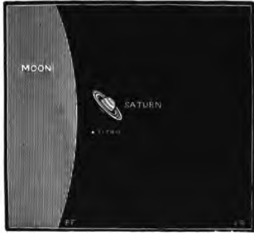
FIG. 36.—OCCULTATION OF SATURN BY THE MOON, APRIL 9, 1883
