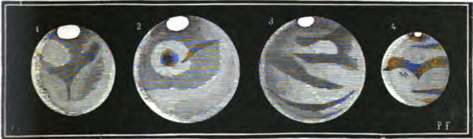
FIG. 169.—TELESCOPIC ASPECT OF MARS ON JULY 30, AUGUST 22, SEPTEMBER 14, AND OCTOBER 26, 1877
