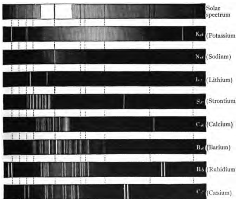
FIG. 144.—COMPARATIVE FIGURE OF SPECTRA
