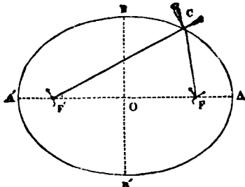
FIG. 8.—THE ELLIPSE
