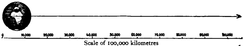
FIG. 12.—DISTANCE TRAVELLED BY THE EARTH IN ONE HOUR RELATIVELY TO ITS DIAMETER
