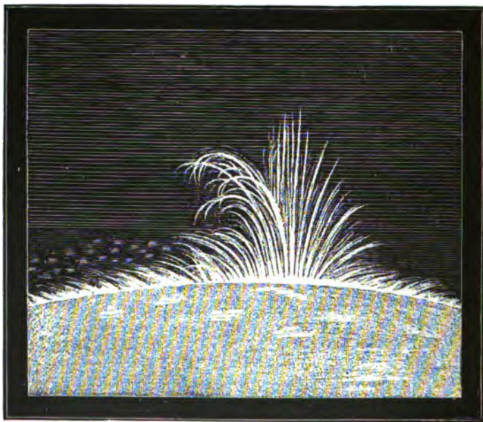
FIG. 116.—AN EXPLOSION IN THE SUN
