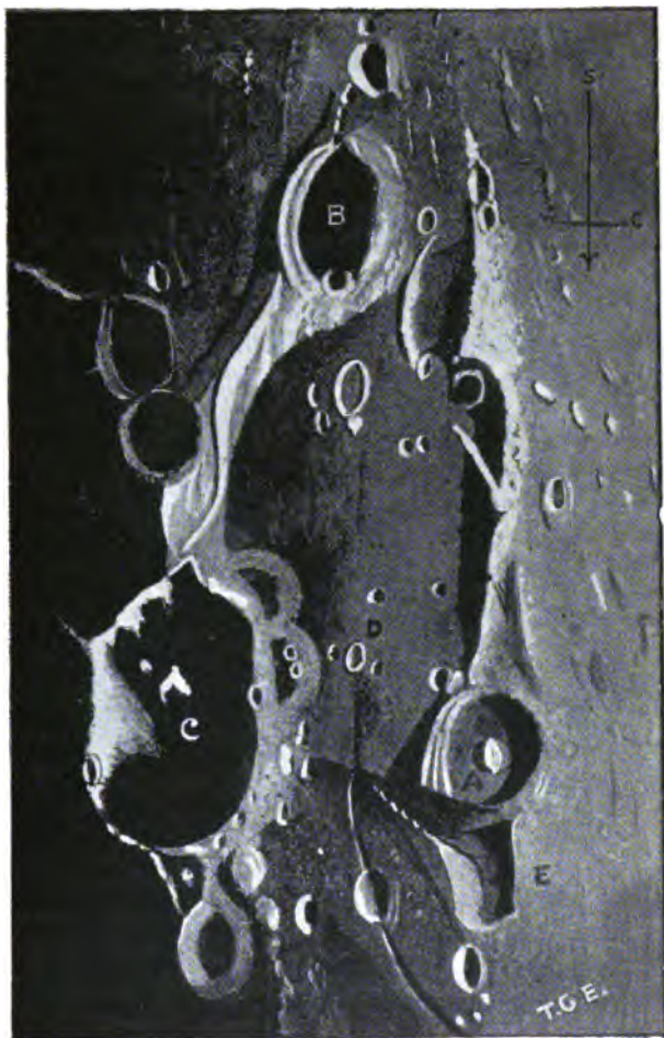
FIG. 57.—VENDELINUS, DECEMBER 17, 1891; 9 HOURS TO 9 HOURS 30 MINUTES. (Drawn by T. G. Elger)
