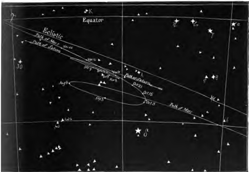
FIG. 146.—PATHS OF MARS AND SATURN DURING THE AUTUMN OF 1877
