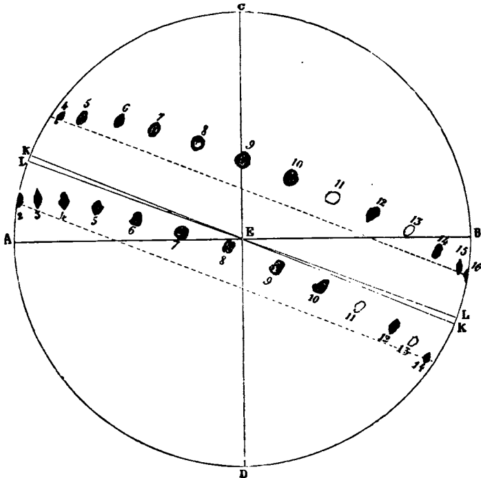
FIG. 104.—ROTATION OF THE SUN, CARRYING WITH IT TWO SPOTS (From a Drawing made in 1627)
