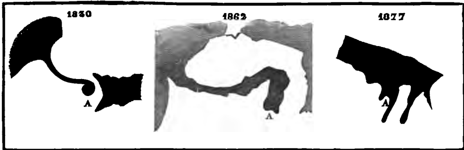
FIG. 171.—PROBABLE VARIATIONS IN THE SEAS ON MARS: HERSCHEL'S STRAIT II. IN 1830, 1862, AND 1877
