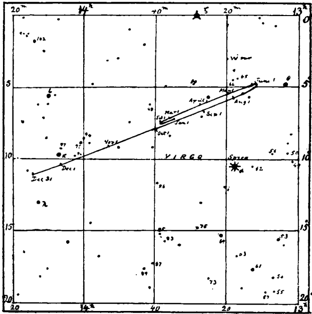
FIG. 148.—APPARENT PATH OF SATURN IN 1894.
