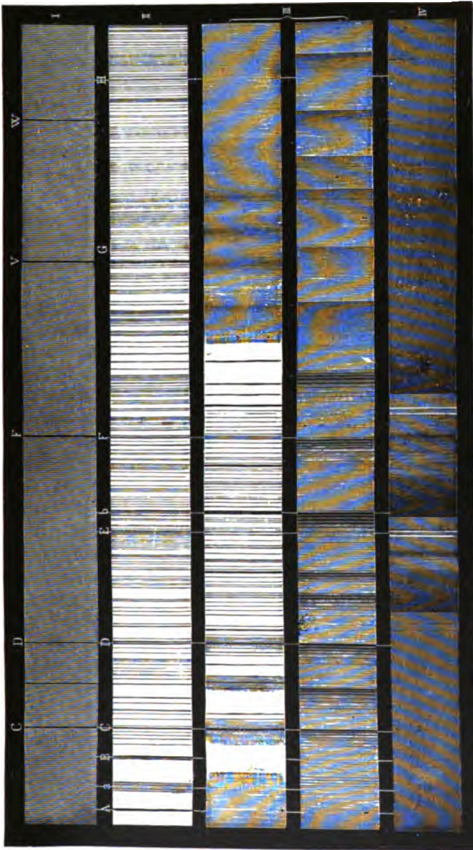
FIG. 263.—PRINCIPAL TYPES OF STELLAR SPECTRA
