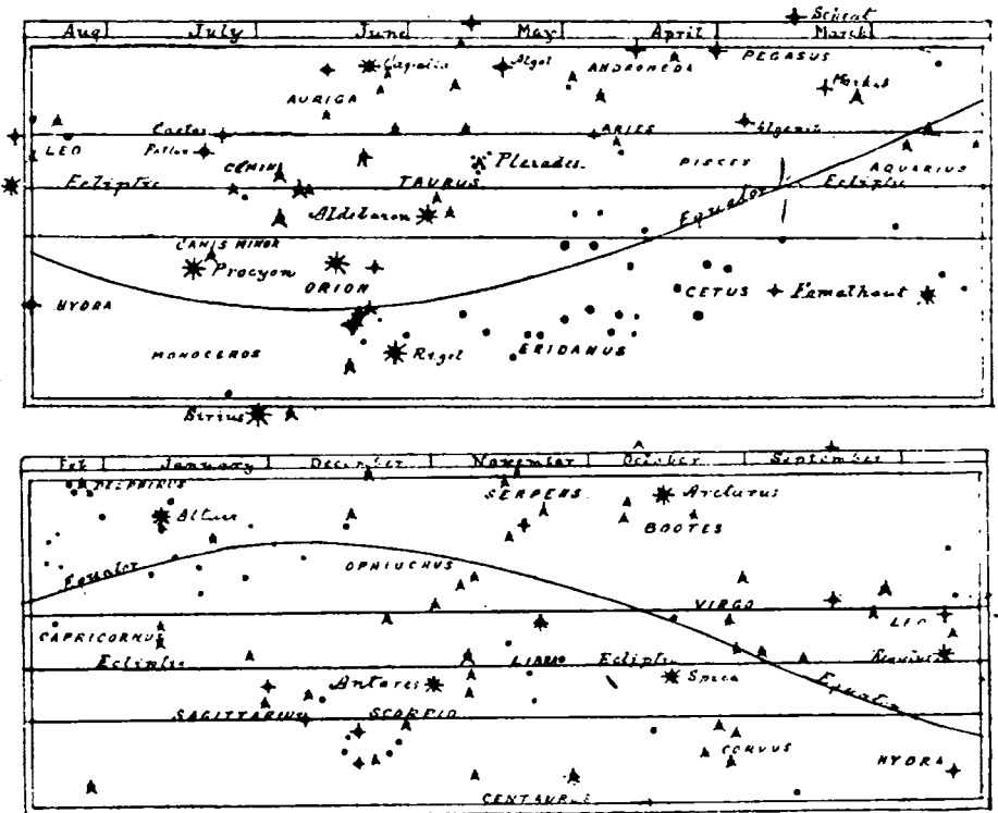
FIG. 18.—PRINCIPAL STARS AND CONSTELLATIONS OF THE ZODIAC
