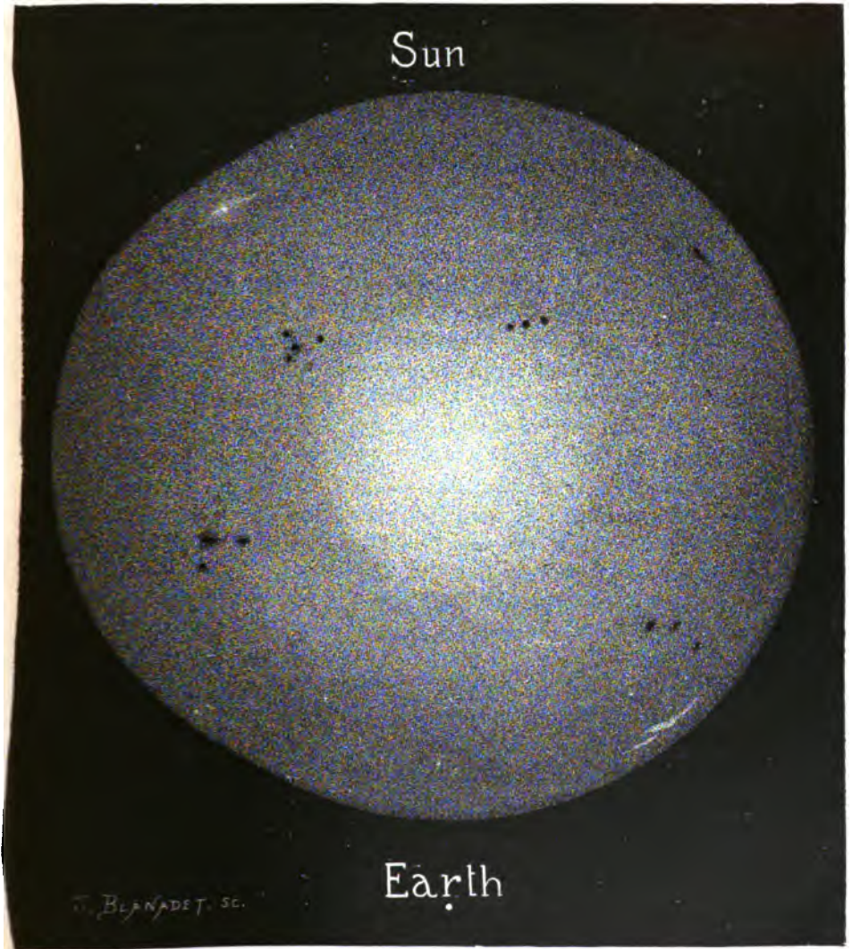
FIG. 22.—COMPARATIVE MAGNITUDES OF THE SUN AND OF THE EARTH
