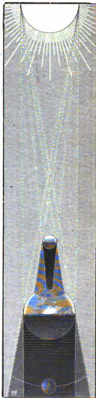
FIG. 66.—THEORY OF ECLIPSES
