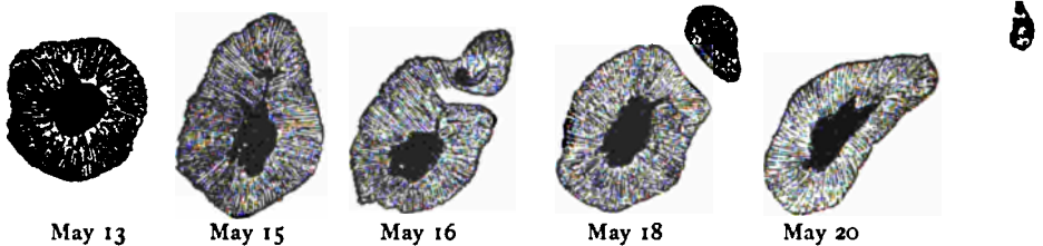
FIG. 107.—SEGMENTATION OF A SUN-SPOT
