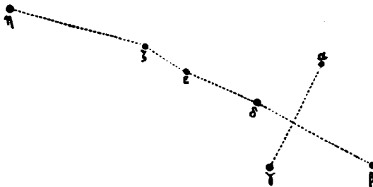
FIG. 270.—THE GREAT BEAR 50,000 YEARS AGO
