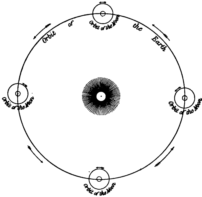
FIG. 78.—ORBITS OF THE EARTH AND OF THE MOON
