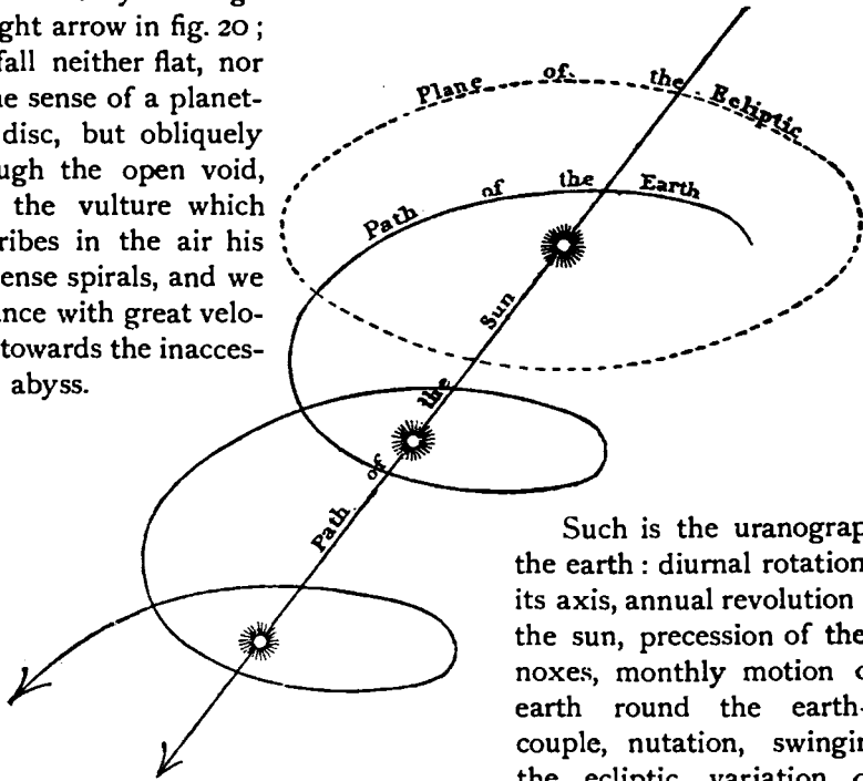
FIG. 20.—SPIRAL COURSE OF THE EARTH IN SPACE
