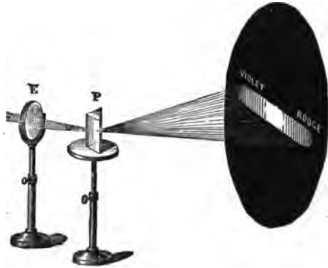
FIG. 140.—PASSAGE OF LIGHT THROUGH A PRISM
