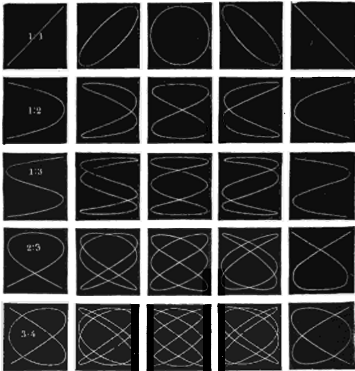
FIG. 88.—GEOMETRY OF MUSIC
