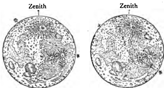
FIG. 54.—OCCULTATION OF STARS BY THE MOON
