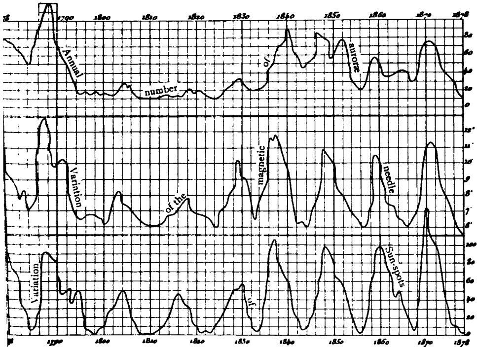
FIG. 130.—ANNUAL VARIATION OF THE AURORA BOREALIS, OF THE MAGNETIC NEEDLE, AND OF SUN-SPOTS DURING A CENTURY
