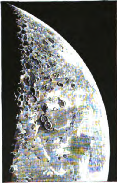
FIG. 45.—LUNAR CRESCENT, SIX DAYS AFTER NEW MOON
