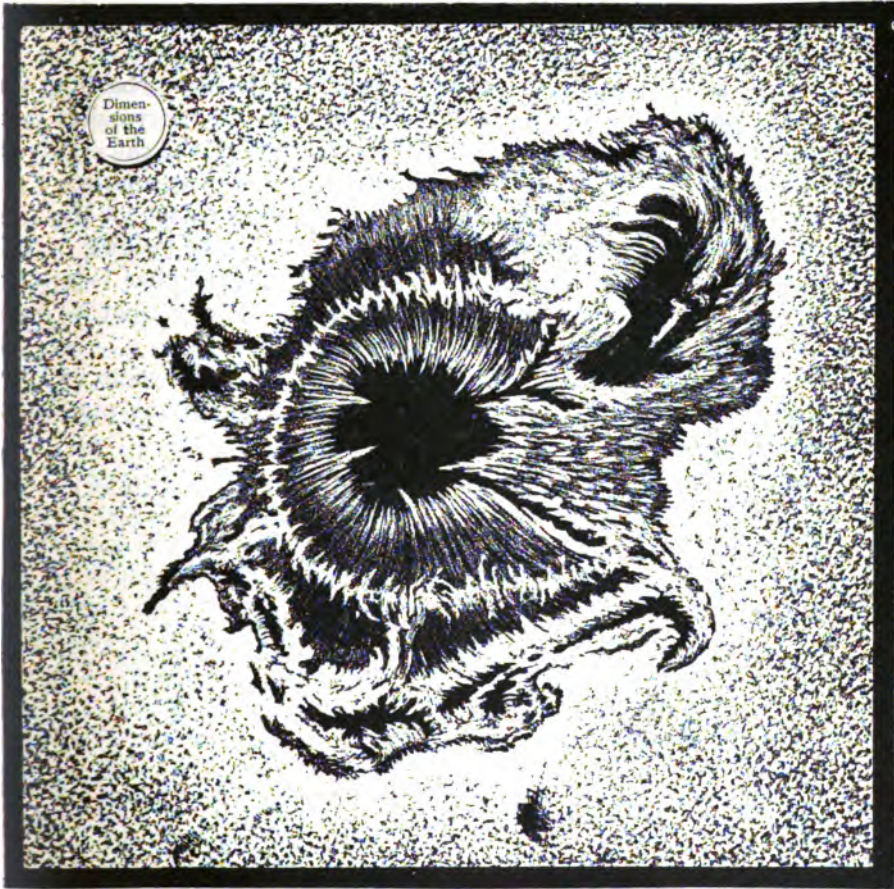
FIG. 105.—ONE OF THE LARGEST SUN-SPOTS: SEVEN TIMES THE SIZE OF THE EARTH. OBSERVED OCTOBER 14, 1883. VISIBLE TO THE NAKED EYE
