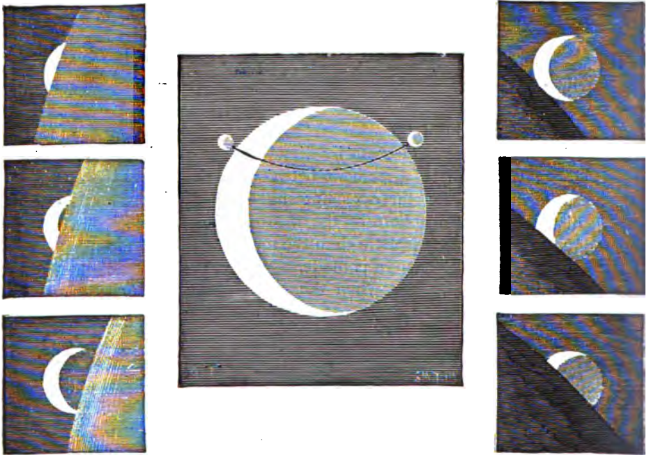
FIG. 55.—OCCULTATION OF VENUS BY THE MOON, OCTOBER 14, 1874
