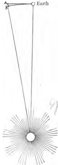
FIG. 96. — MEASURING THE SUN'S ATTRACTION
