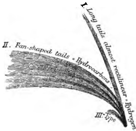
FIG. 229.—THEORY OF VARIOUS COMETARY TAILS
