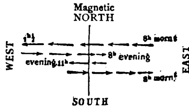
FIG. 128.—MOVEMENTS OF THE MAGNETIC NEEDLE
