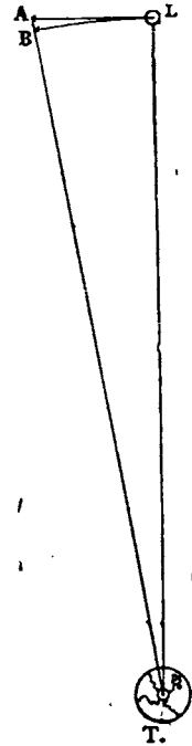
FIG. 34.—EXPLANATION OF THE MOVEMENT OF THE MOON
