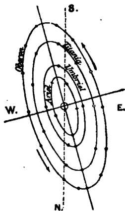
FIG. 196. — INCLINATION OF THE SYSTEM OF URANUS, SEEN FROM THE EARTH
