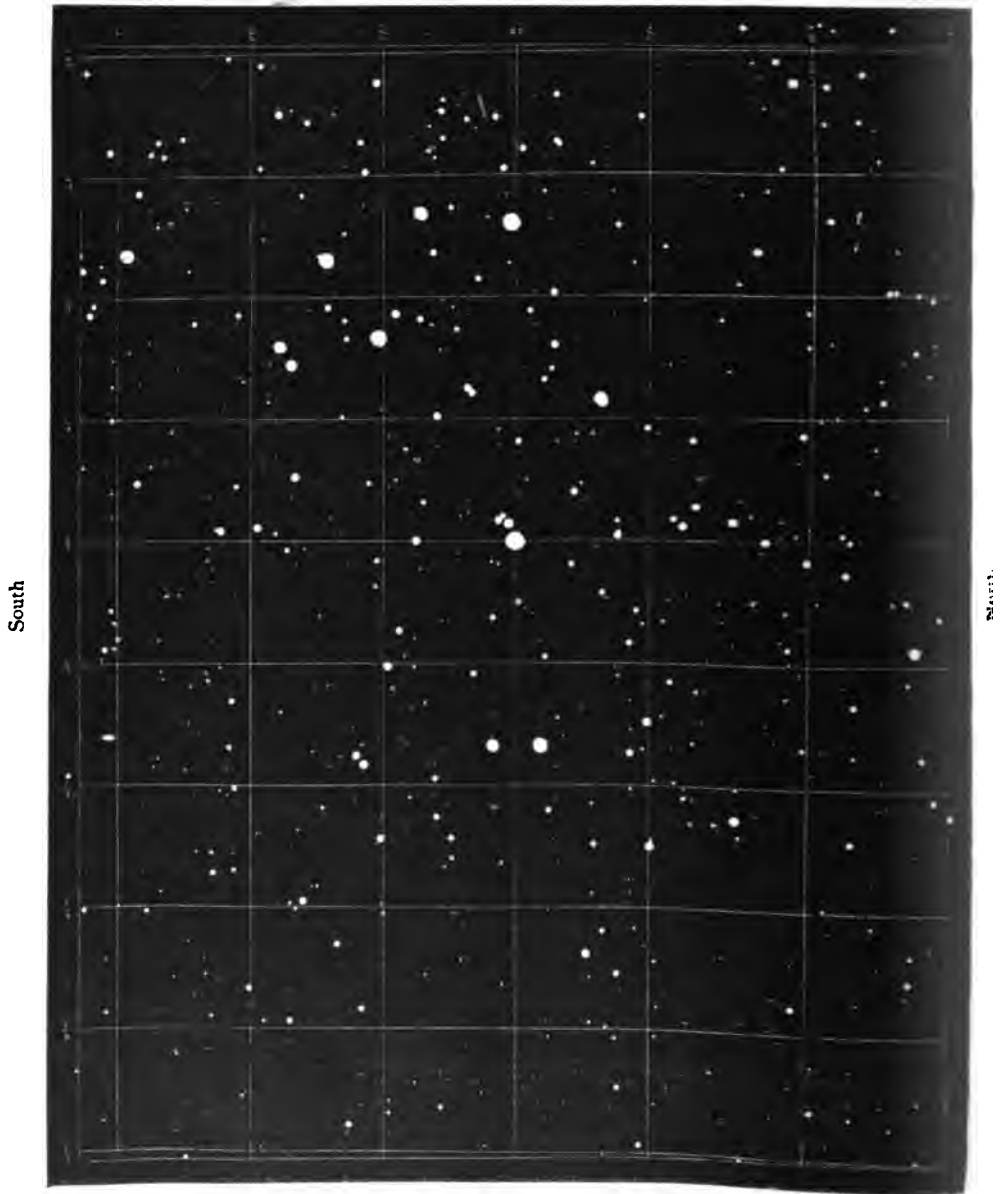
FIG. 278.—THE PLEIADES AS SEEN IN THE TELESCOPE
