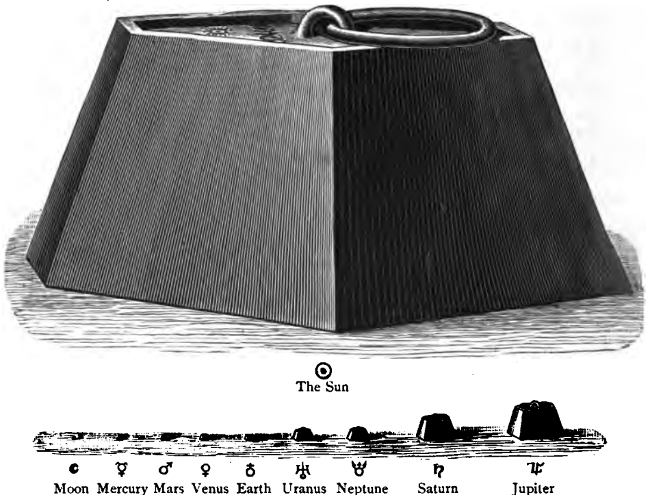
FIG. 97.—WEIGHTS REPRESENTING THE MASSES OF THE CELESTIAL BODIES
