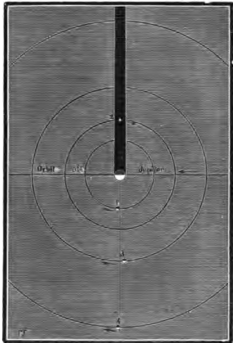
FIG. 184.—DISAPPEARANCE OF JUPITER'S SATELLITES
