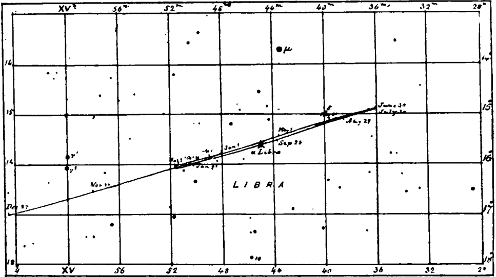
FIG. 149.—APPARENT PATH OF URANUS IN 1894
