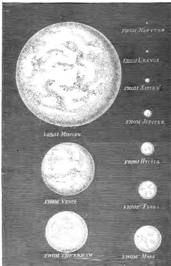
FIG. 198.—PROPORTIONAL SIZE OF THE SUN AS SEEN FROM DIFFERENT PLANETS
