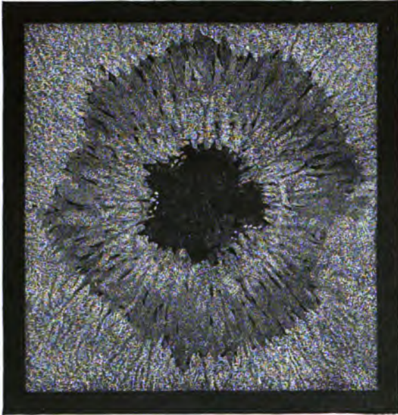
FIG. 106.—TYPE OF AN ORDINARY SUN-SPOT
