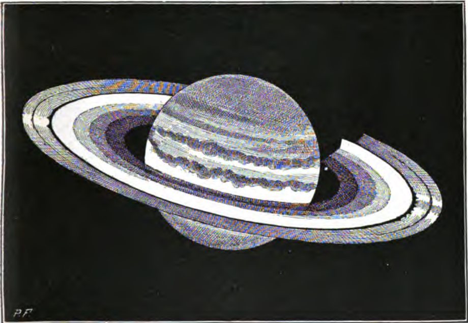
FIG. 191.—TELESCOPIC ASPECT OF SATURN IN 1874
