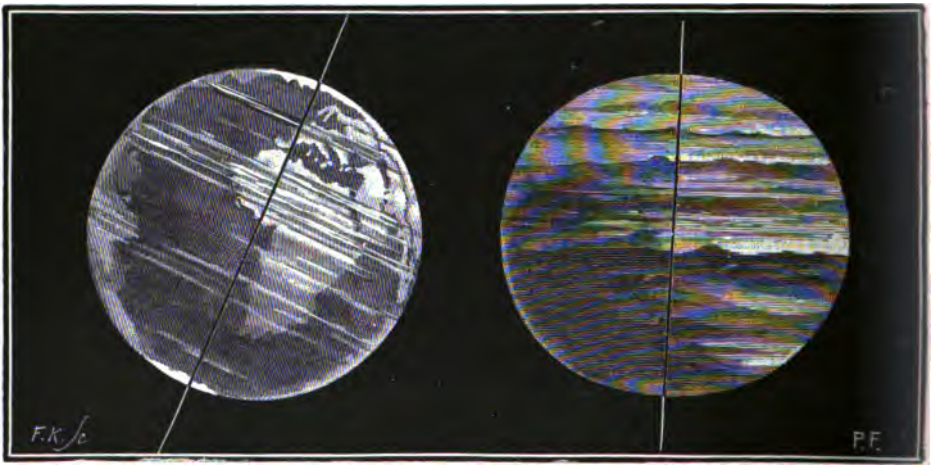
FIG. 176.—COMPARATIVE INCLINATION OF THE AXIS OF THE EARTH AND OF THAT OF JUPITER
