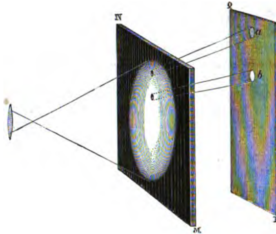
FIG. 98.—VARIATIONS OF LUMINOUS INTENSITY OF THE SOLAR DISC
