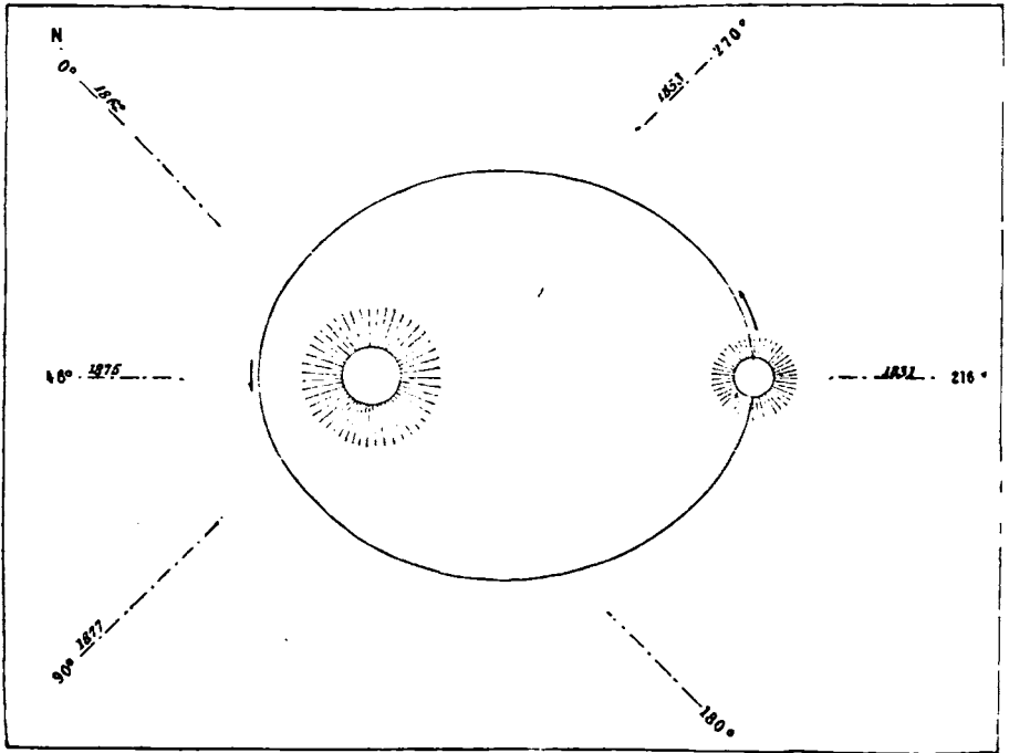
FIG. 136.—SYSTEM OF THE DOUBLE SUN ALPHA CENTAURI
