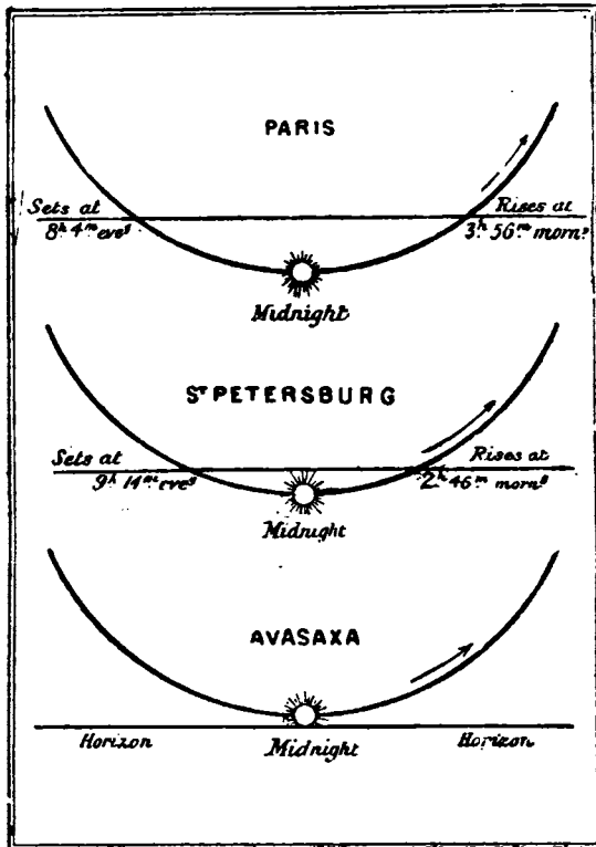
FIG. 10.—THE SUN AT MIDNIGHT, ON JUNE 21, FOR PARIS, ST. PETERSBURG, AND MOUNT AVASAXA
