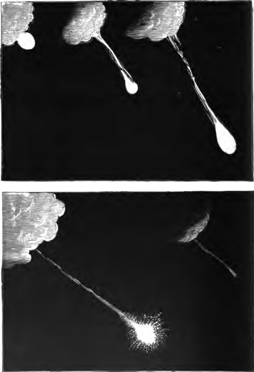
FIG. 238.—FIREBALL EMERGING FROM BEHIND A CLOUD, NOVEMBER 23, 1877, 8 h 24 m . (Drawn by J. Plant)
