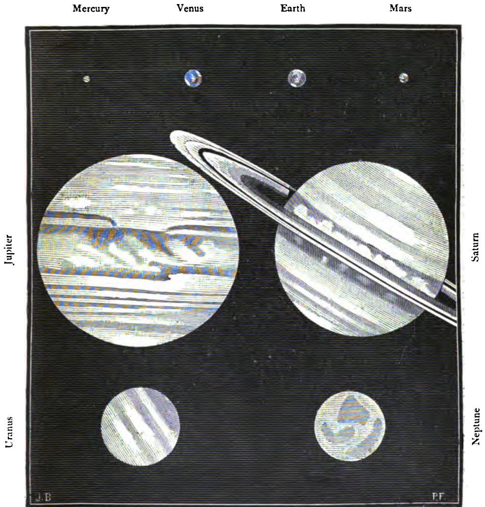
FIG. 175.—THE PRINCIPAL WORLDS OF THE SOLAR SYSTEM
