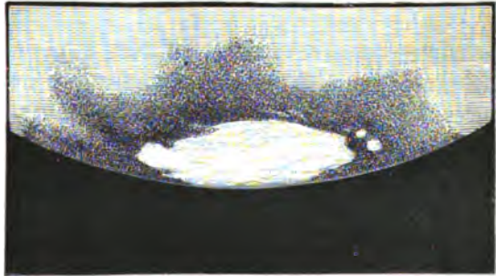
FIG. 170.—THE SOUTH POLE OF MARS
