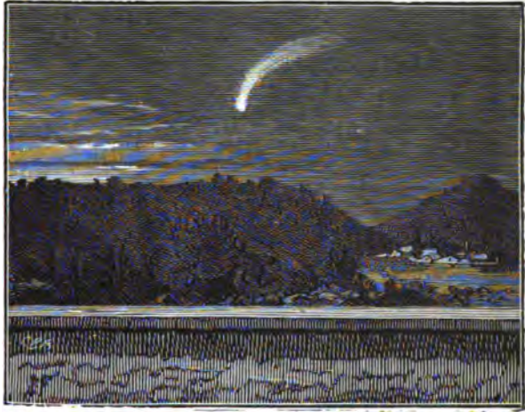
FIG. 205.—THE COMET OF 1853
