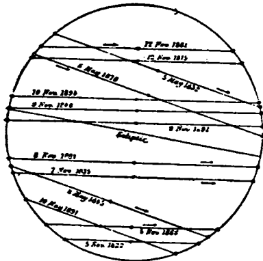
FIG. 156.—TRANSITS OF MERCURY IN THE NINETEENTH CENTURY
