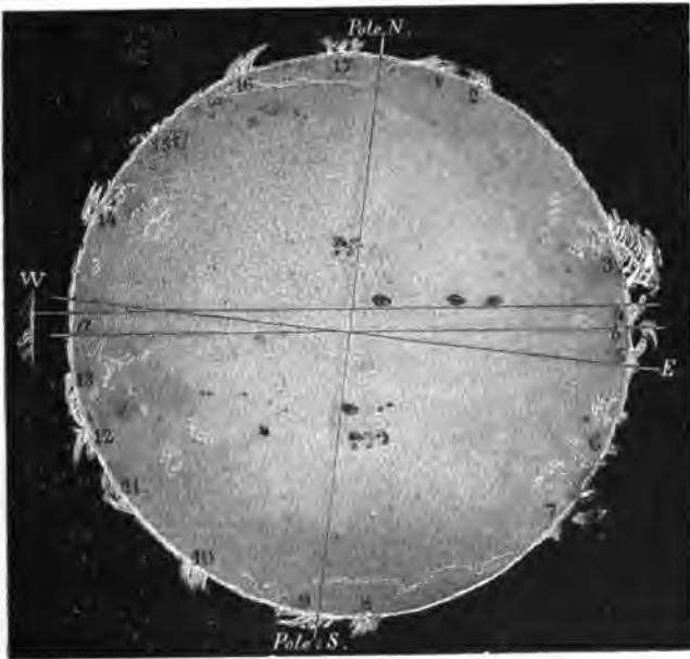
FIG. 115.—PROMINENCES OBSERVED JULY 23, 1871
