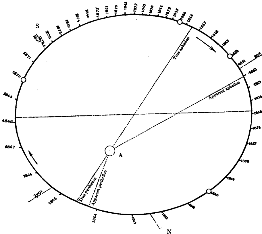
FIG. 267.—APPARENT ORBIT OF THE DOUBLE STAR ζ HERCULIS AS SEEN FROM THE EARTH
