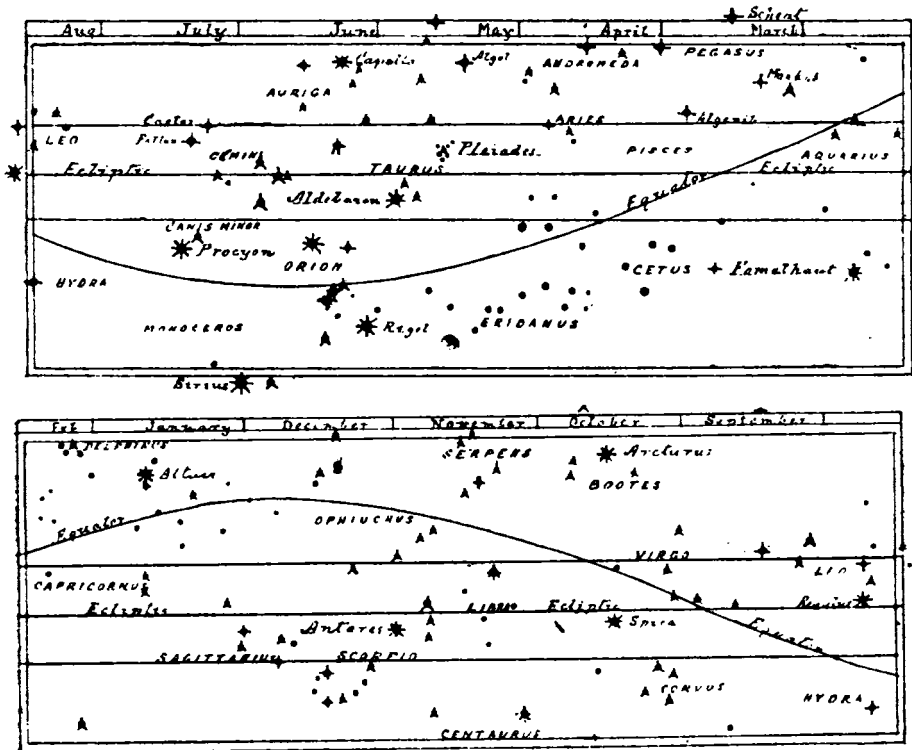
FIG. 250.—PRINCIPAL STARS AND CONSTELLATIONS OF THE ZODIAC
