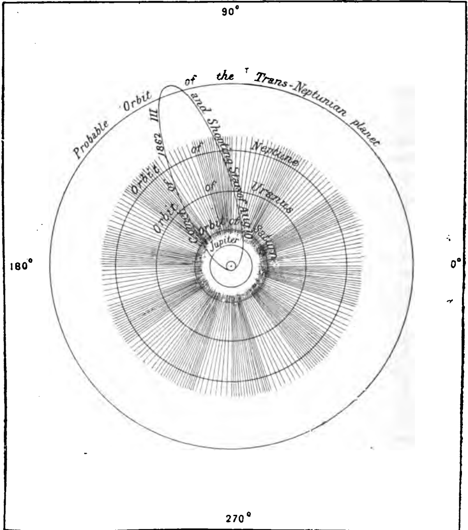
FIG. 202.—DIAGRAM SHOWING THE PROBABLE EXISTENCE OF A TRANS-NEPTUNIAN PLANET AT FORTY-EIGHT TIMES THE DISTANCE OF THE EARTH FROM THE SUN
