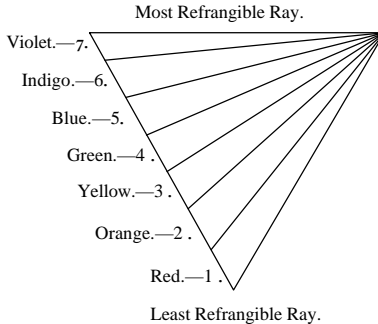
Fig. 33. PRISMATIC SPECTRUM.
